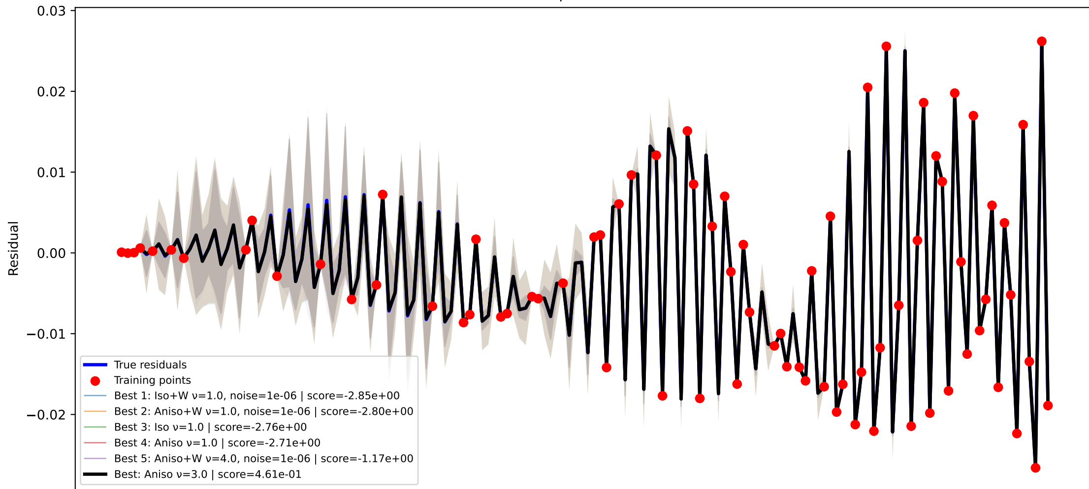
GPR kernel comparison node=41 RMSE=8.057e-05, train RMSE=1.876e-11
